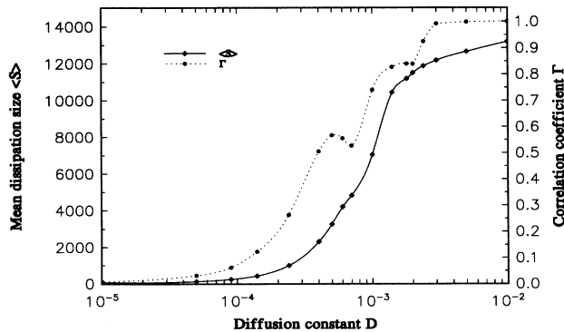
FIG. 2. Variation of the mean dissipation size \langle S \rangle (solid line) and the correlation coefficient \Gamma (dashed line) against the diffusion constant D . All the simulations are done in a 64 \times 64 lattice with E_{c1} = 5.0 and E_{c2} = 2.0 , respectively. The same set of parameters is used in Figs. 3 and 4.
